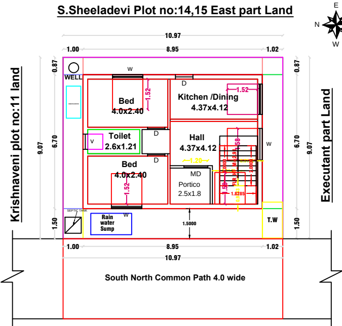
SITE PLAN CUM GROUND FLOOR PLAN
