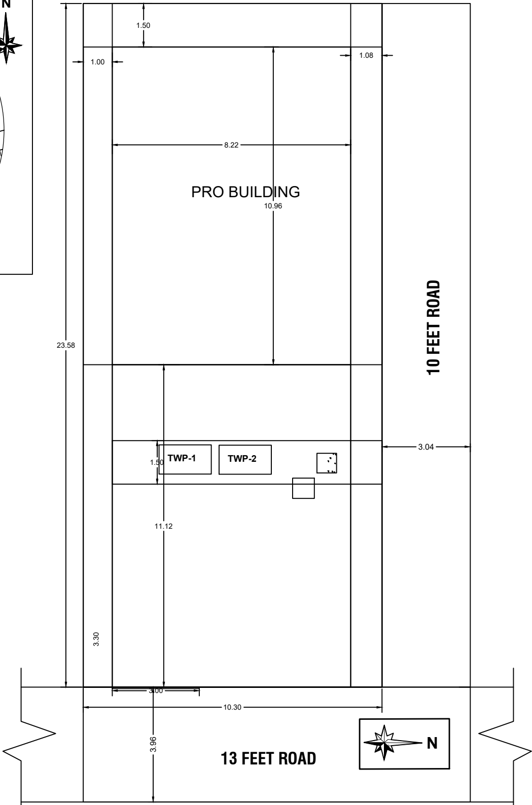
SITE PLAN
