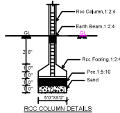
RCC COLUMN DETAILS
