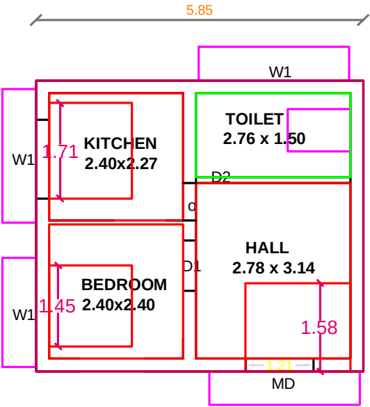
GROUND FLOOR PLAN PROPOSED
