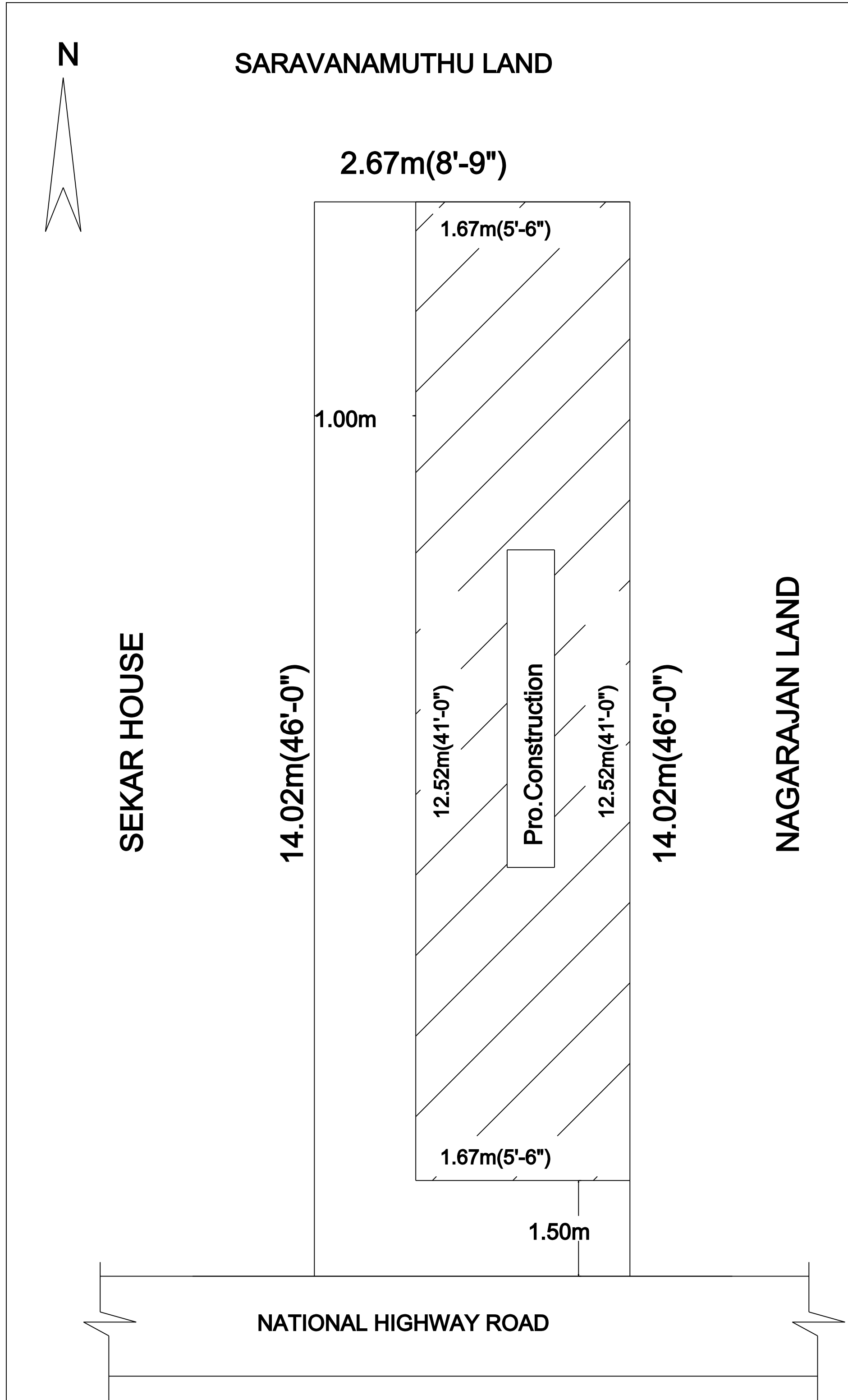
SITE PLAN
