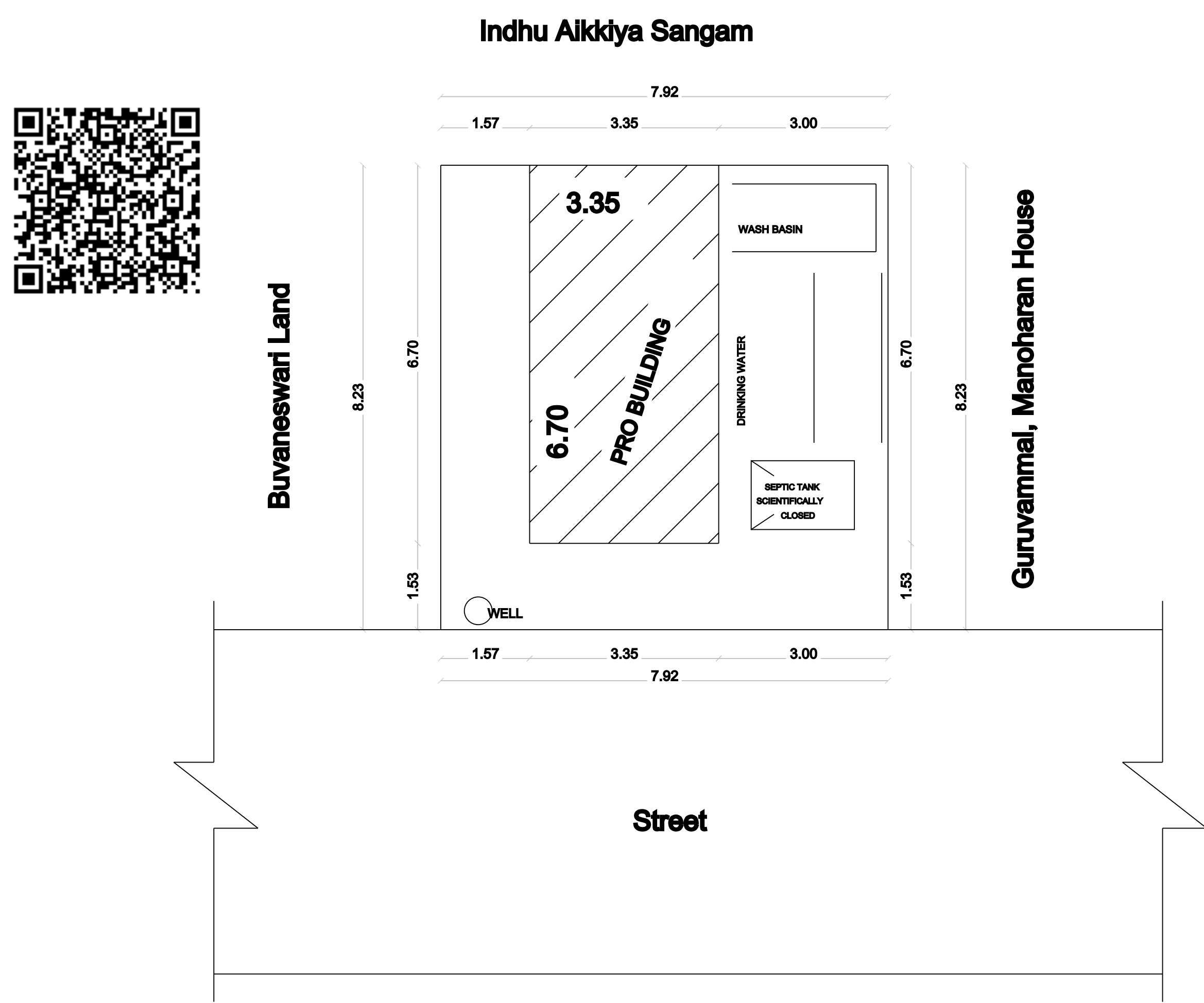
SITE PLAN & KEY PLAN
