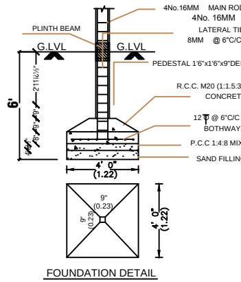
FOUNDATION DETAIL
