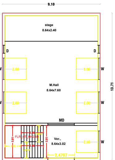
PRO. GROUND FLOOR PLAN
