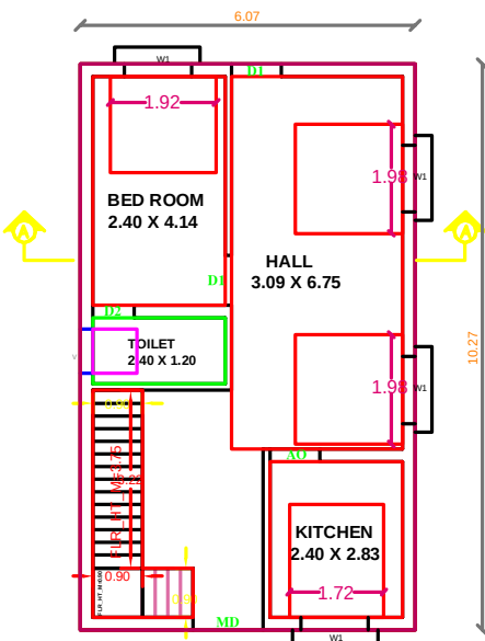
GROUND FLOOR PLAN PROPOSED
