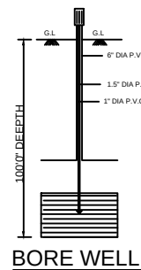
BORE WELL
