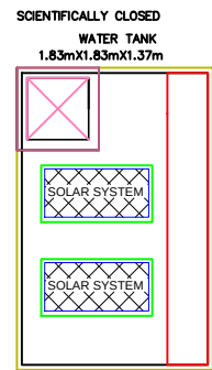
TERRACE FLOOR PLAN
