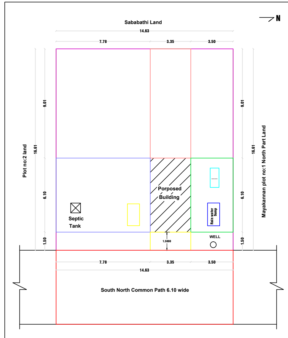
SITE PLAN CUM KEYPLAN
