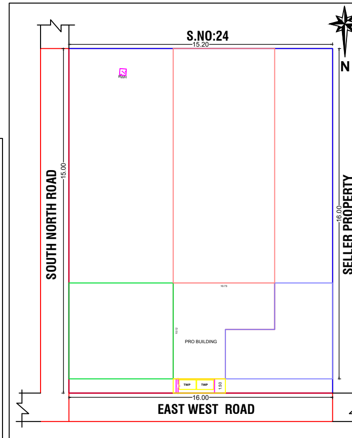
SITE PLAN
