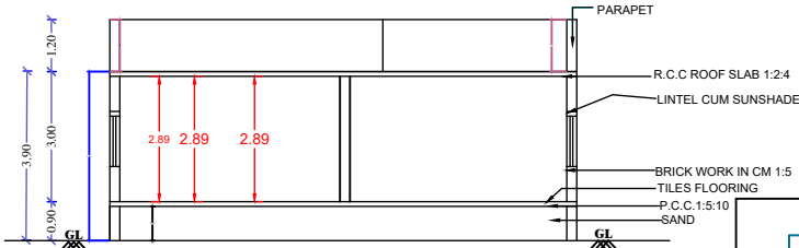
SECTION ON A-B
