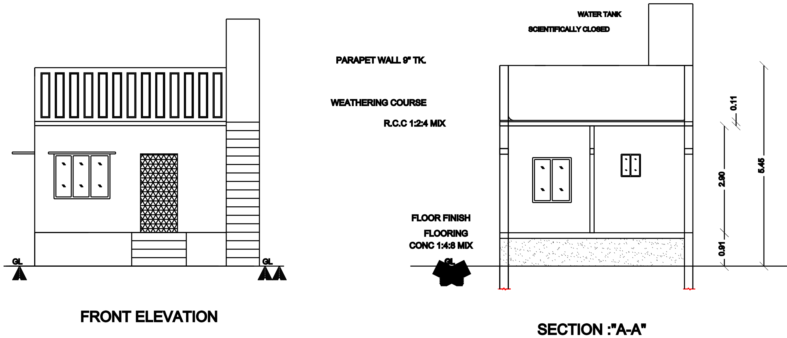
SECTION : "A-A"
