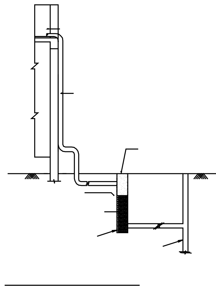
PERCULATION PIT
