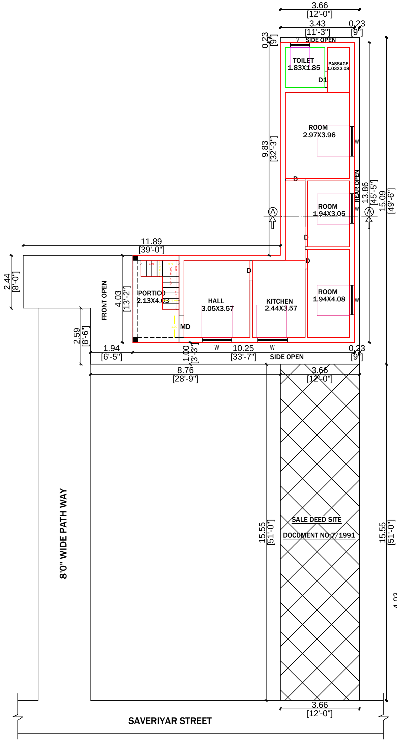
PRO. GROUND FLOOR PLAN
