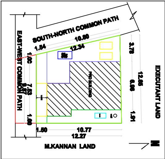
SITE PLAN & KEY PLAN (1:100)
