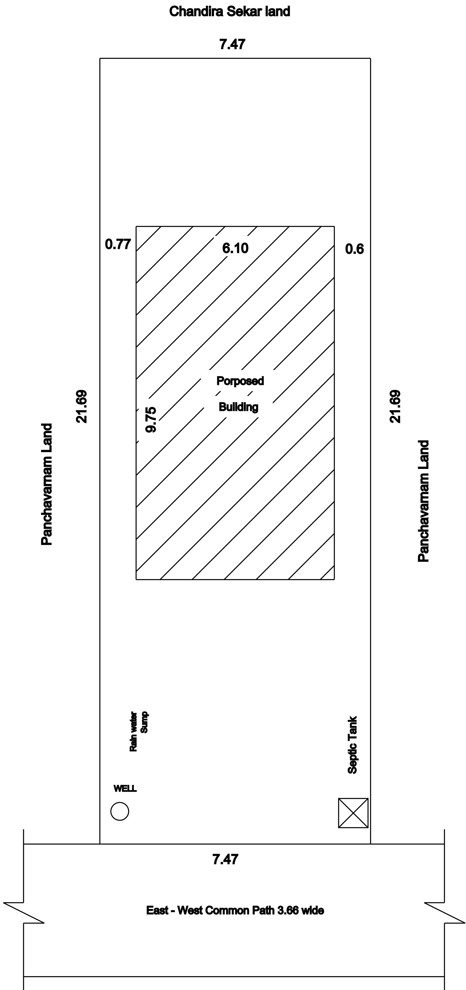
SITE PLAN CUM KEYPLAN
