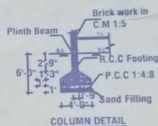
COLUMN DETAIL
