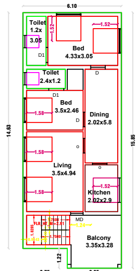
PORPOSED FIRTS FLOOR PLAN
