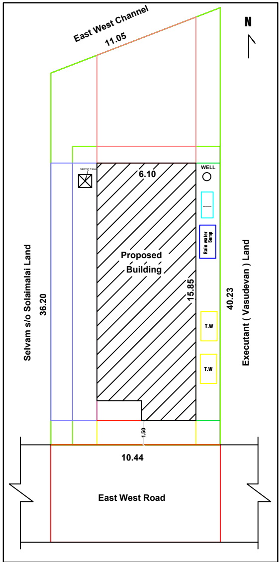
SITE PLAN & KEY PLAN (1:100)
