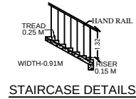
STAIRCASE DETAILS
