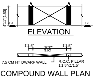
ELEVATION COMPOUND WALL PLAN
