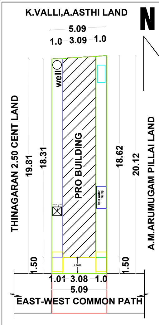
SITE PLAN & KEY PLAN
