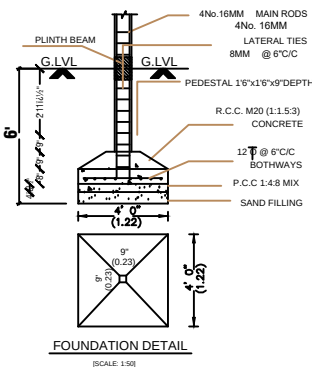
FOUNDATION DETAIL
