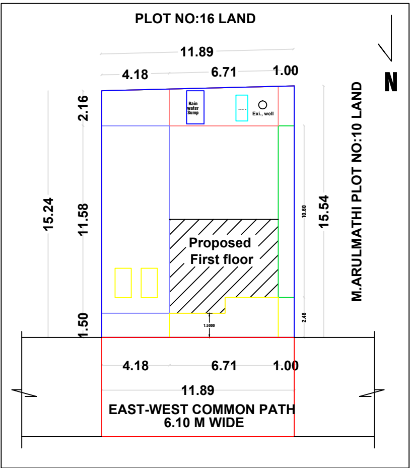
SITE PLAN & KEY PLAN (1:100)
