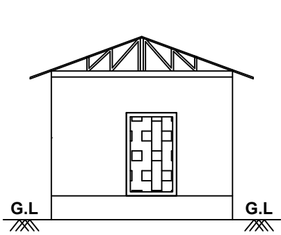
FRONT ELEVATION "A"
