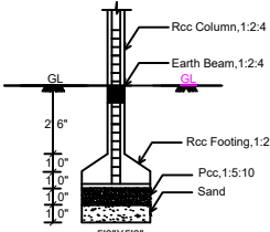
RCC COLUMN DETAILS
