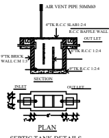
SEPTIC TANK DETAILS
