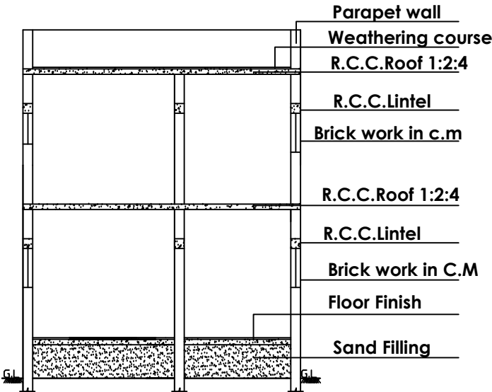
SECTION AN AA
