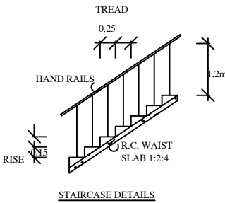
STAIRCASE DETAILS
