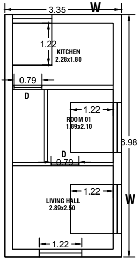
PRO., GROUND FLOOR PLAN
