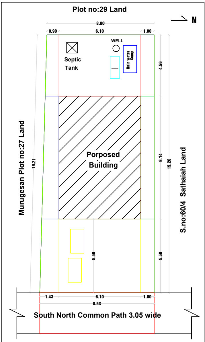
SITE PLAN CUM KEYPLAN
