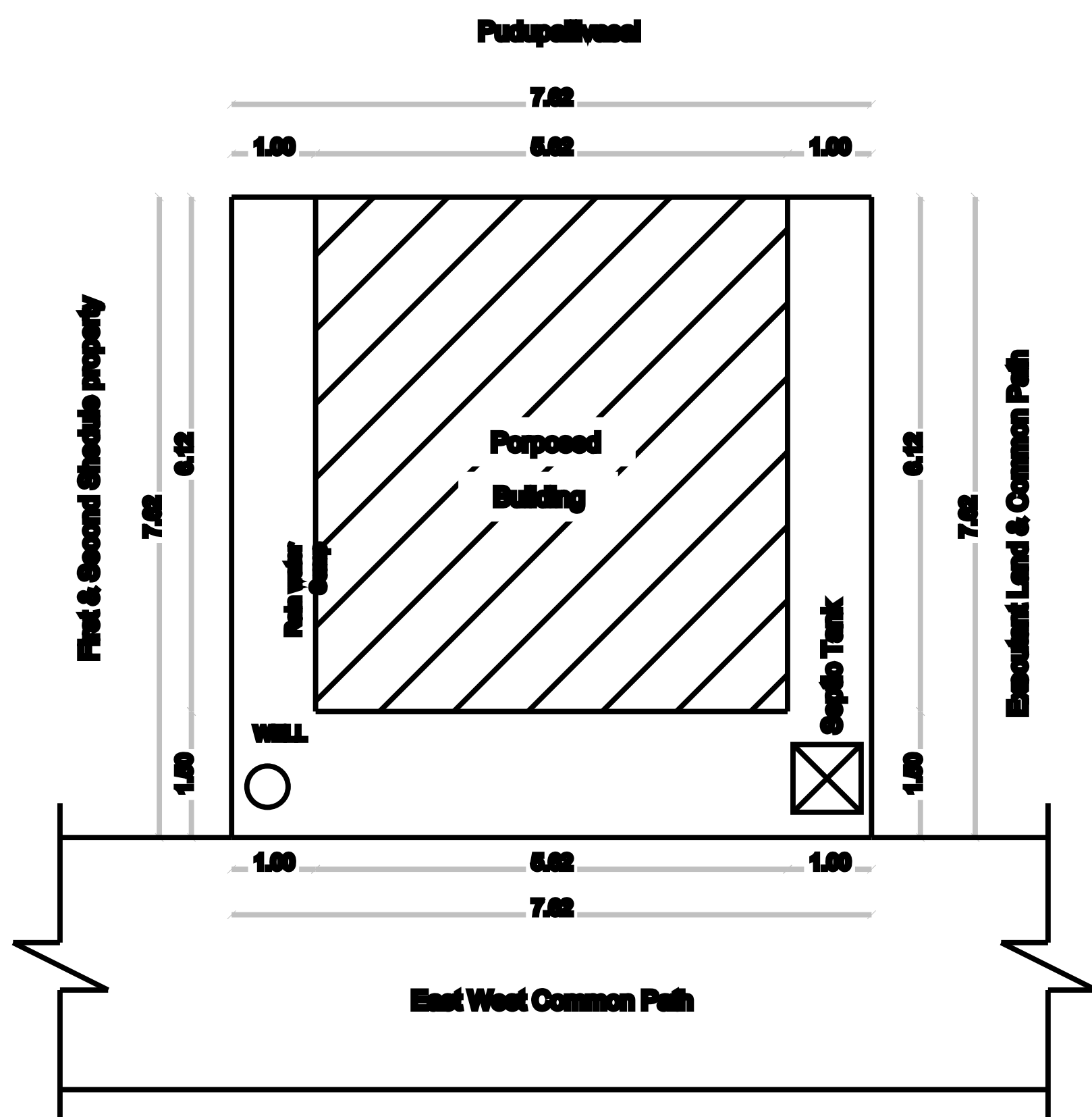
SITE PLAN CUM KEYPLAN
