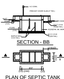
PLAN OF SEPTIC TANK
