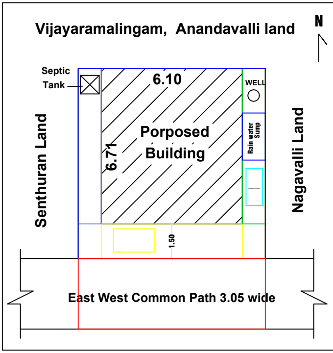
SITE PLAN CUM KEYPLAN
