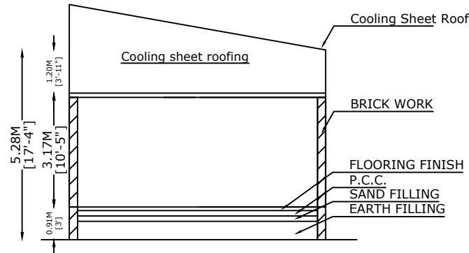
SECTION ON XX
