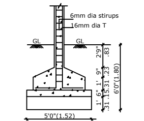
COLUMN FOUNDATION DETAIL
