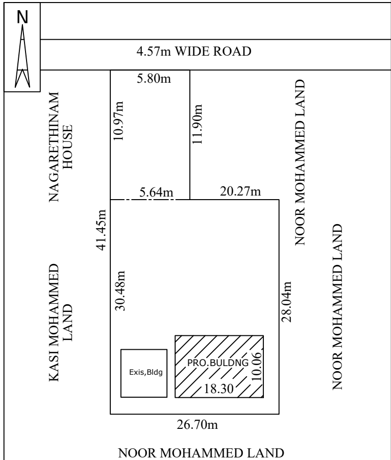
SITE PLAN
