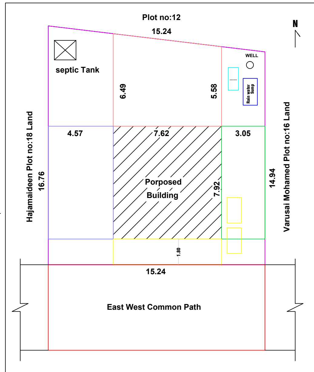
SITE PLAN CUM KEYPLAN
