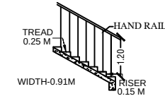
STAIRCASE DETAILS
