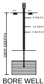
BORE WELL
