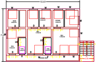
PRO., FIRST FLOOR PLAN
