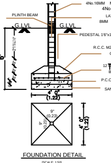
FOUNDATION DETAIL (SCALE: 1:50)
