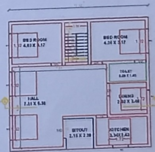
GROUND FLOOR PLAN PROPOSED
