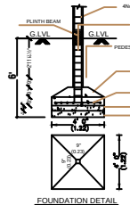
FOUNDATION DETAIL
