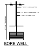
BORE WELL
