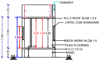
SECTION ON A-B
