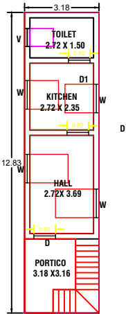
PRO., GROUND FLOOR PLAN
