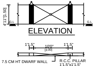
ELEVATION COMPOUND WALL PLAN
