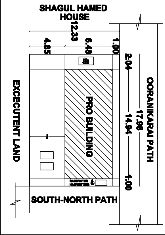
SITE PLAN & KEY PLAN (1:100)
