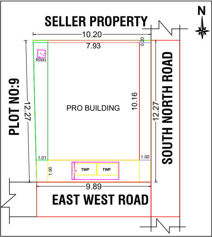
SITE PLAN
