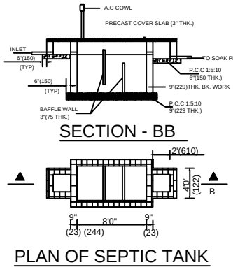
PLAN OF SEPTIC TANK
