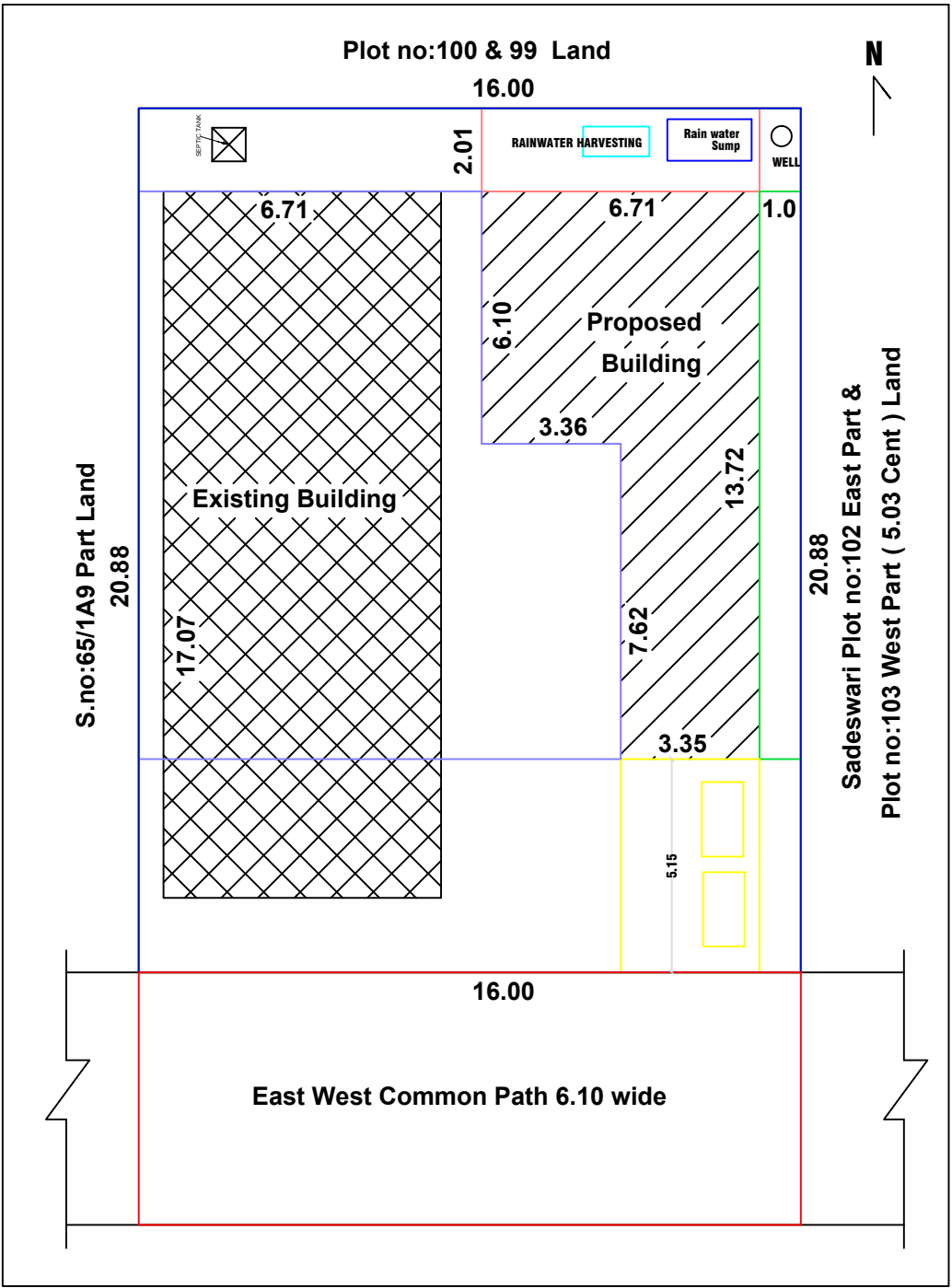
SITE PLAN & KEY PLAN (1:100)
