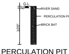
PERCOLATION PIT
