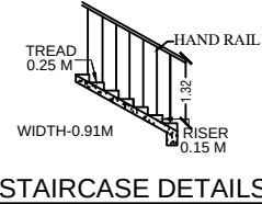
STAIRCASE DETAILS
