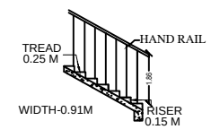
STAIRCASE DETAILS
