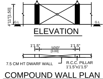
COMPOUND WALL PLAN
