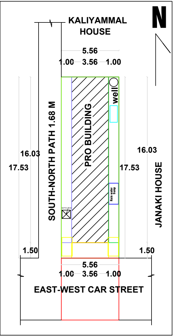
SITE PLAN & KEY PLAN
