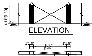
COMPOUND WALL PLAN
