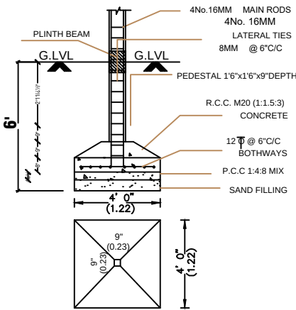
FOUNDATION DETAIL
