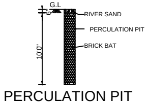
PERCOLATION PIT
