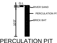
PERCOLATION PIT
