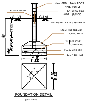
FOUNDATION DETAIL
