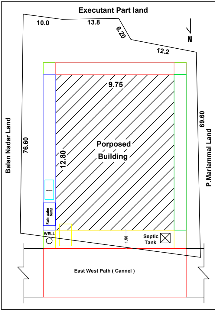
SITE PLAN CUM KEYPLAN
