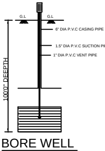
BORE WELL
