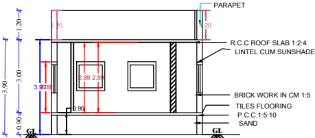
SECTION ON A-E
