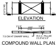
ELEVATION COMPOUND WALL PLAN
