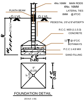
FOUNDATION DETAIL (SCALE 1:50)
