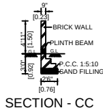
SECTION - CC
