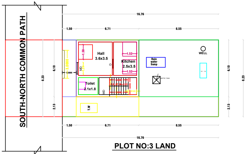
SITE PLAN CUM GROUND FLOOR PLAN
