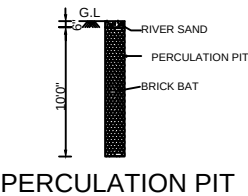
PERCOLATION PIT
