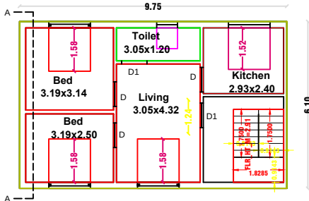
PORPOSED FIRTS FLOOR PLAN
