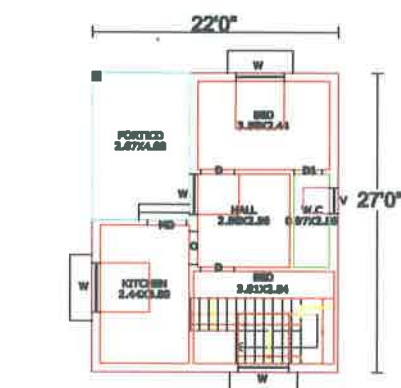
EXIST.GROUND FLOOR PLAN
