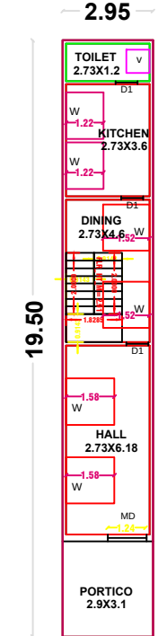
GROUND FLOOR
