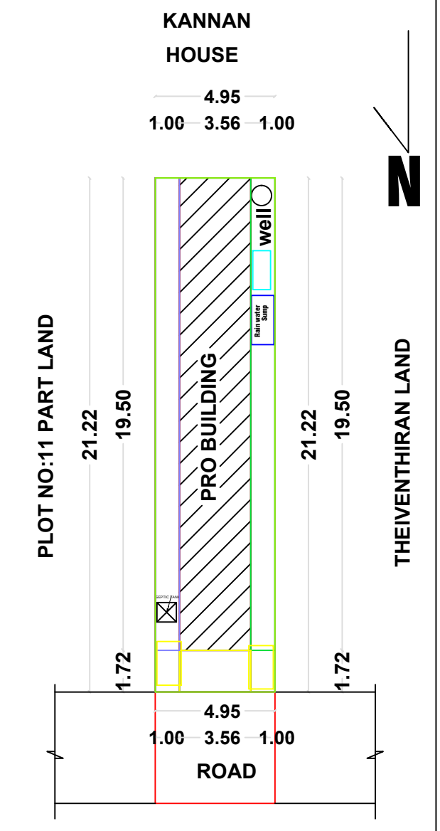
SITE PLAN & KEY PLAN
