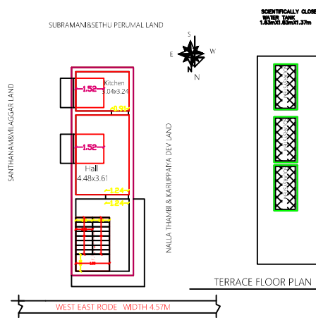
SITE PLAN CUM GROUND FLOOR PLAN
