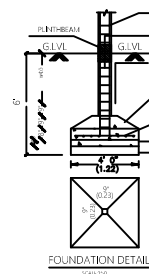
FOUNDATION DETAIL
