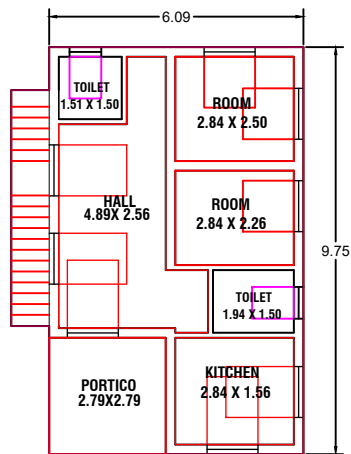
PRO., GROUND FLOOR PLAN
