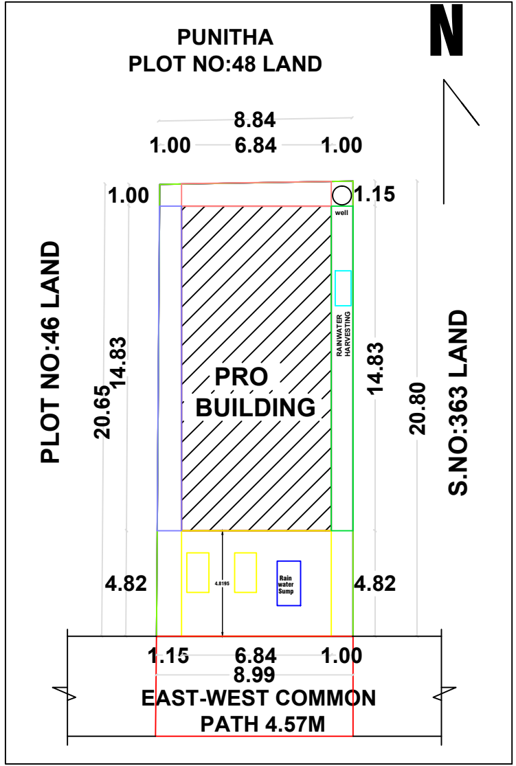
SITE PLAN & KEY PLAN (1:100)
